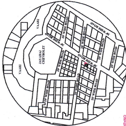
TOPO PLAN 1:3200
