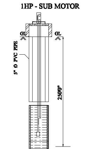
BOREWELL DETAILS
