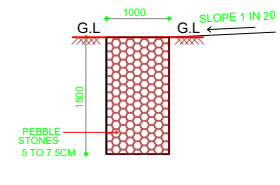
SECTION OF PEBBLE TRENCH
