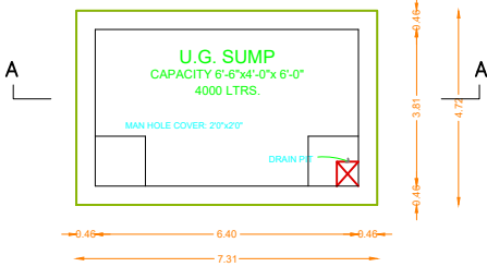
SUMP DETAIL
