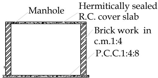
Section On 'Y-Y'
