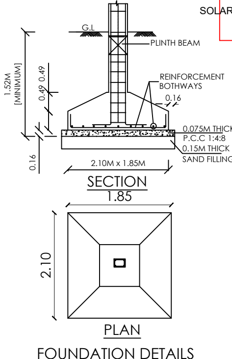
FOUNDATION DETAILS
