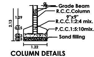
COLUMN DETAILS
