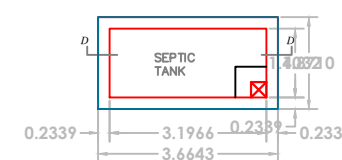
PLAN OF SEPTIC TANK SCALE 1"=2'0"
