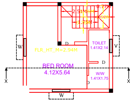
RST FLOOR PLAN
