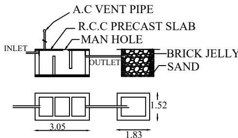
DETAILS OF SEPTIC TANK & DISPERSION TRENCH
