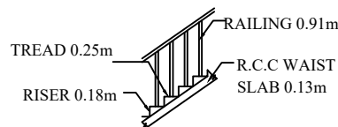
STAIRCASE DETAILS
