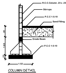
COLUMN DETAIL
