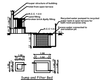
Sump and Filter Bed
