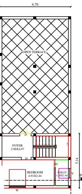
PRO. FIRST FLOOR PLAN
