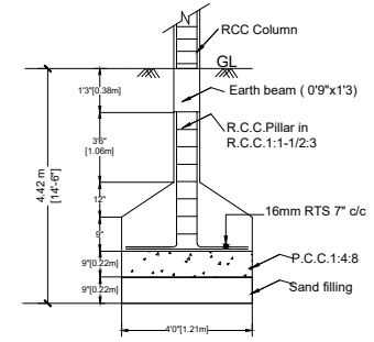
FOUNDATION DETAILS
