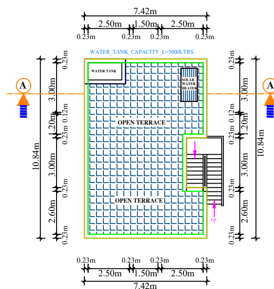
TERRACE PLAN
