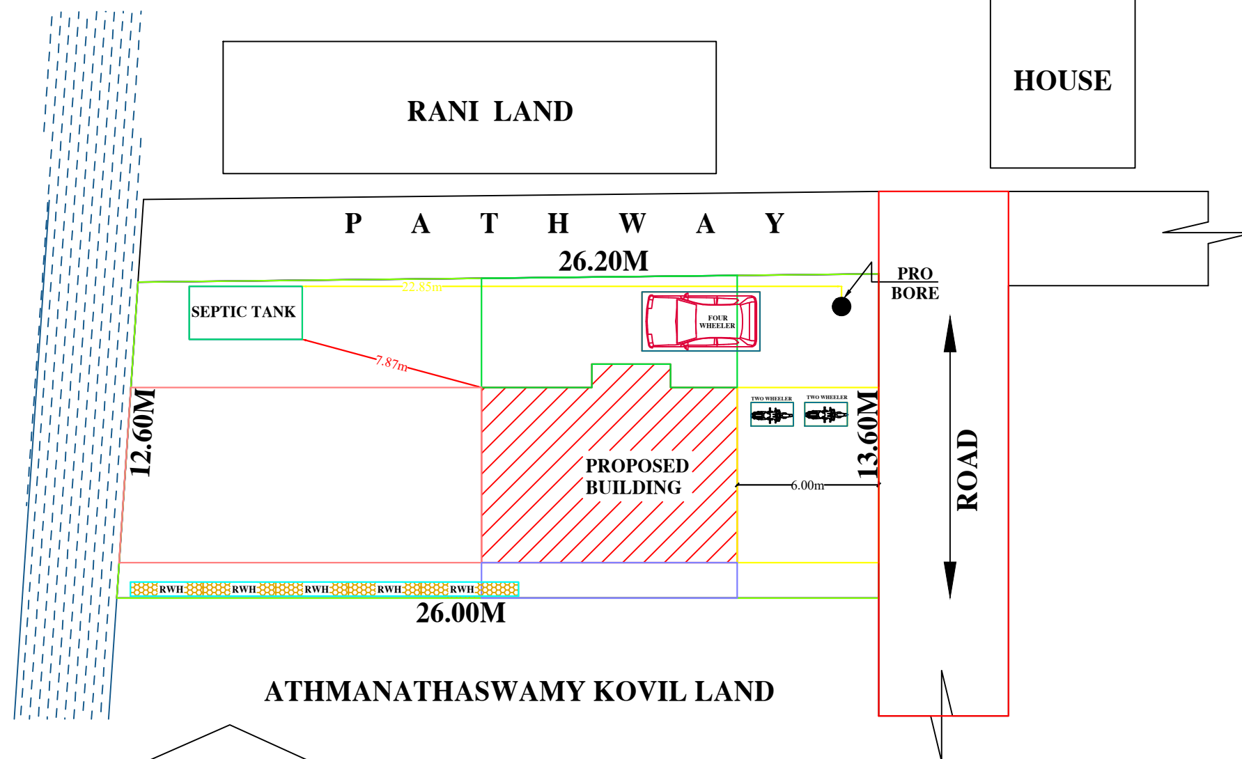
SITE PLAN
