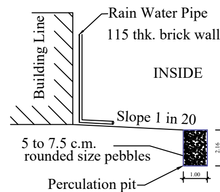
RAIN WATER HARVESTING PERCUSSION PIT RWH_CAPACITY_L=2000LTRS
