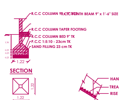
COLUMN DETAILS PLAN
