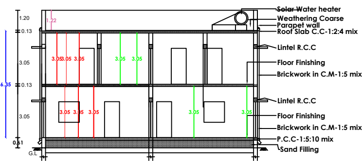
SECTION"AB"
