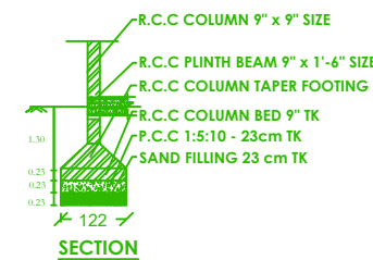
SECTION
