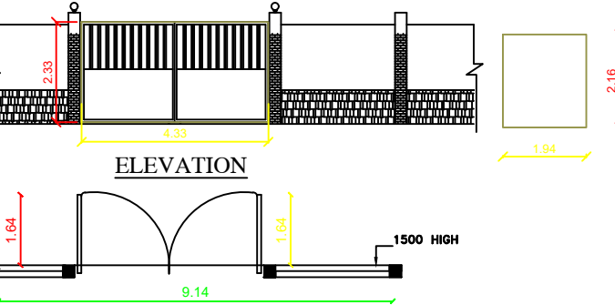
PLAN Compound wall Detail
