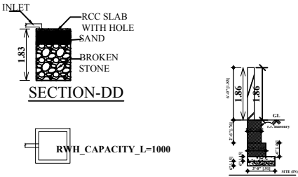
PLAN OF RW H
