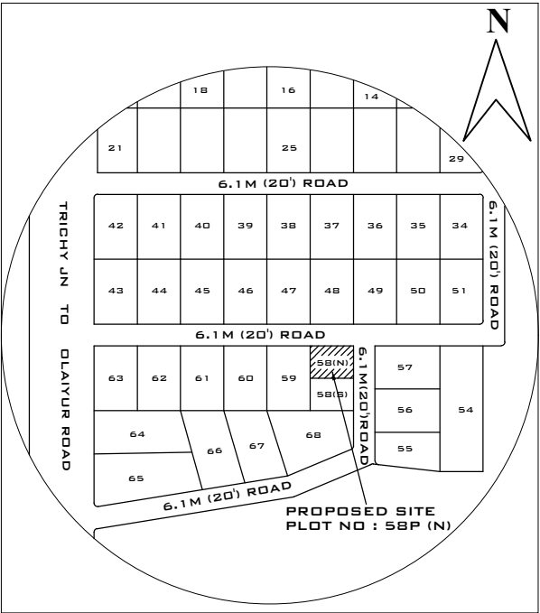
TOPO PLAN (NOT TO SCALE)
