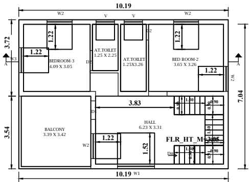
PROPOSED FIRST FLOOR
