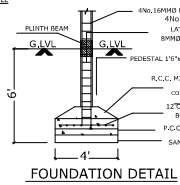
FOUNDATION DETAIL
