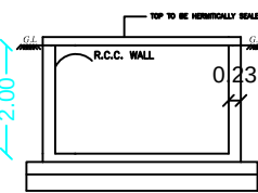
R.C.C. WALL SECTION (SAMPLE)
