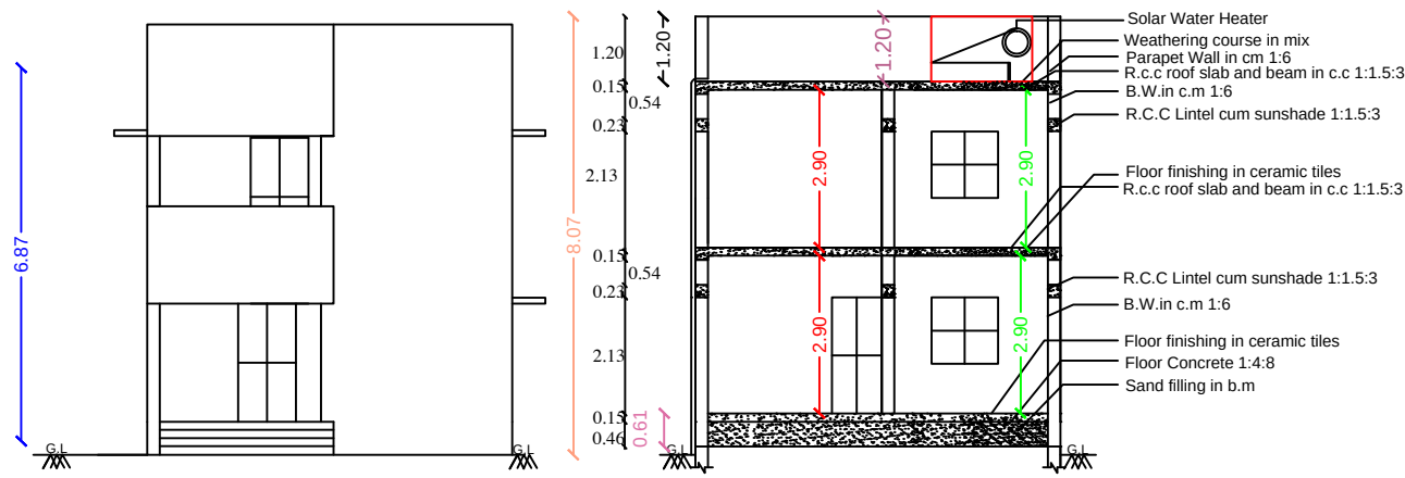
SECTION - "AB - CD "
