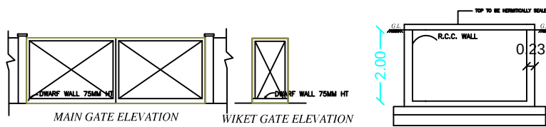
R.C.C. WALL SECTION (SAMPLE)
