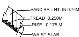
HAND RAIL HT. IN 0.76M
