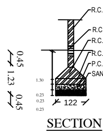
SECTION
