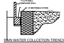
RAIN WATER COLLECTION TRENCH
