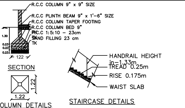
COLUMN DETAILS
