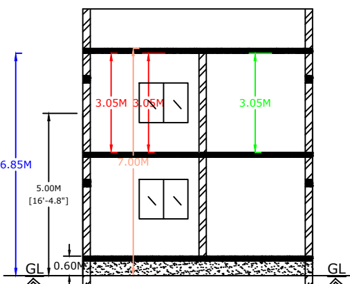
SECTION ON XX
