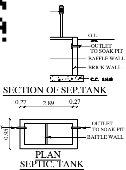
SECTION
