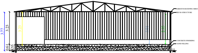
SECTION ON AB
