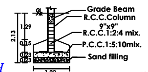
COLUMN DETAILS
