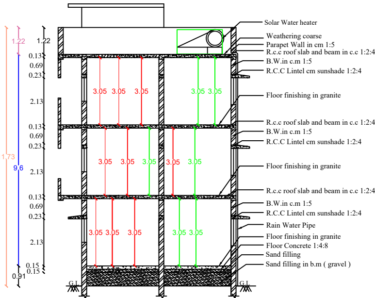
SECTION - "AB,CD"
