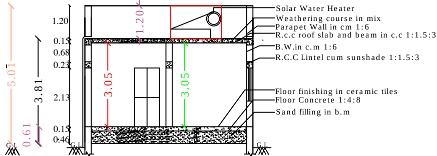
SECTION - "AB "
