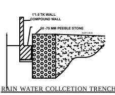
RAIN WATER COLLECTION TRENCH
