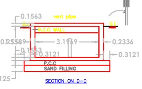
SECTION ON D-D
