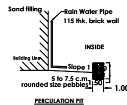
PERCOLATION PIT
