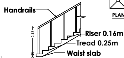
STAIRCASE DETAILS
