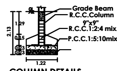
COLUMN DETAILS
