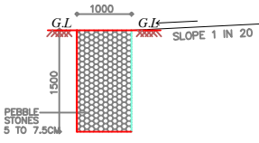
SECTION OF PEBBLE TRENCH
