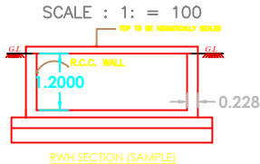
RW SECTION (SAMPLE) RW_CAPACITY_L = 2000LTRS SCALE 1"=2'0"
