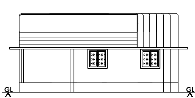
FRONT ELEVATION
