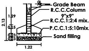
COLUMN DETAILS
