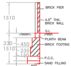
COMPOUND WALL DETAIL PLAN
