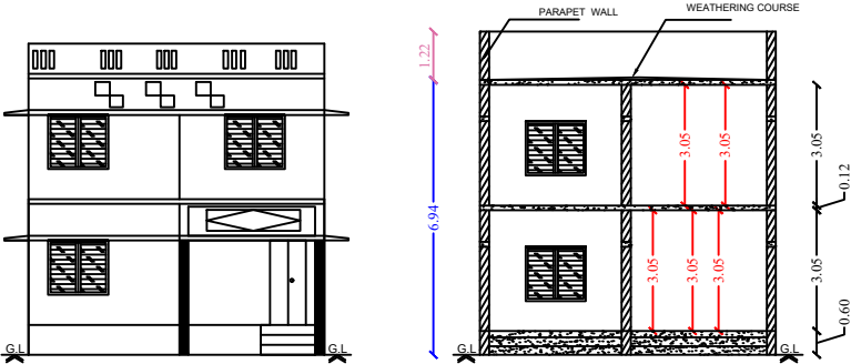
Section on-"AA"
