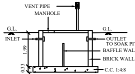
SECTION OF SEP.TANK
