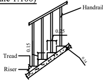
STAIRCASE DETAIL
