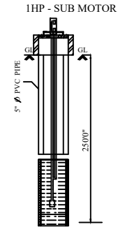
BOREWELL DETAILS
