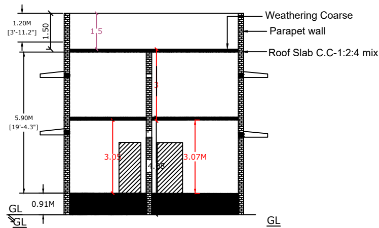
CROSS SECTION ON ABCD
