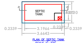
SEPTIC TANK
