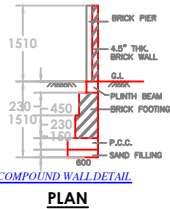
COMPOUND WALL DETAIL
