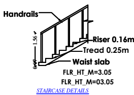
STAIRCASE DETAILS
