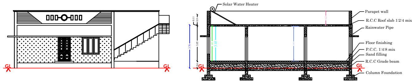
FRONT ELEVATION
