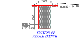
SECTION OF PEBBLE TRENCH
