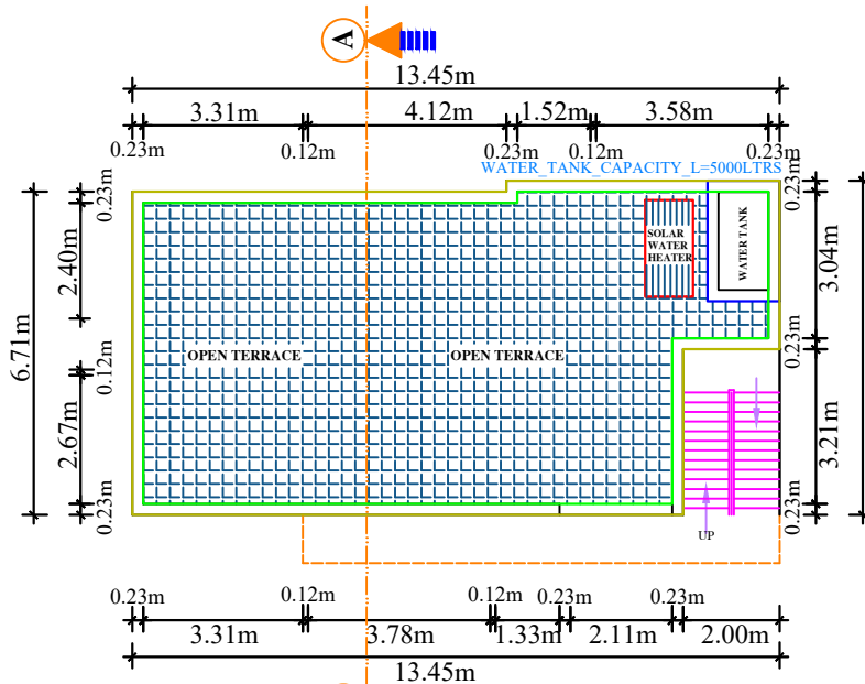
TERRACE PLAN
