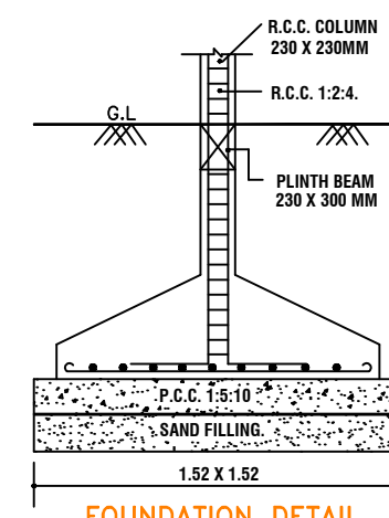
FOUNDATION DETAIL
