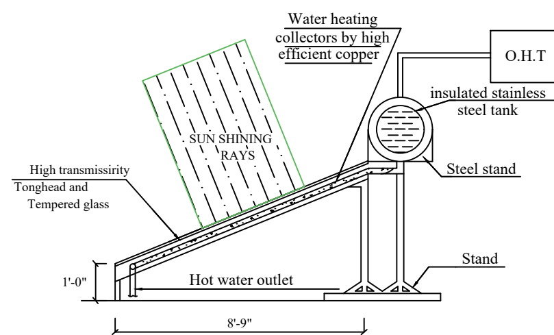
SECTION SOLAR WATER HEATER
