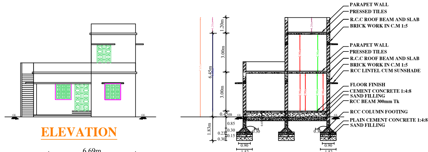
SECTION [A-A]
