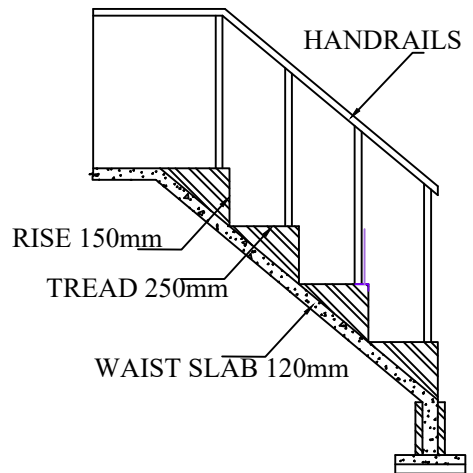
STAIRCASE DETAILS
