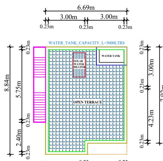
TERRACE PLAN
