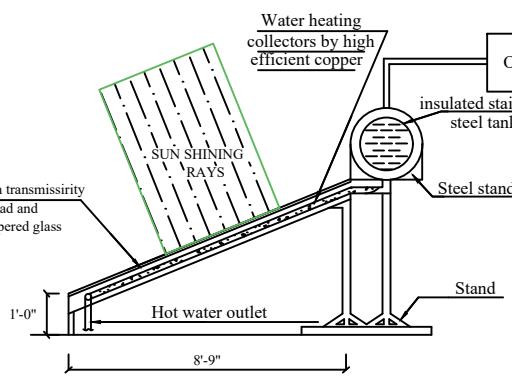
SECTION SOLAR WATER HEATER
