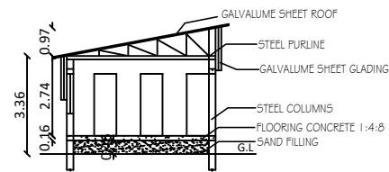
SECTION ON GG
