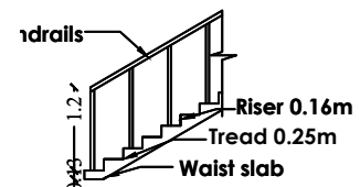
STAIRCASE DETAILS
