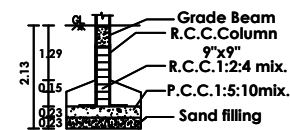
COLUMN DETAILS
