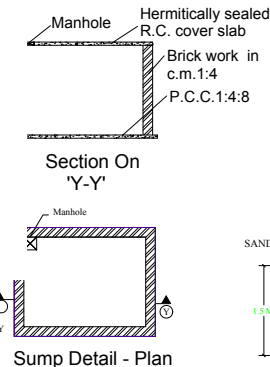
Sump Detail - Plan
