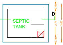
PLAN OF SEPTIC TANK
