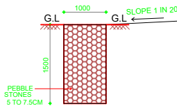
SECTION OF PEBBLE TRENCH SCALE : 1 : 100
