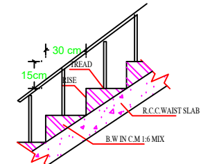
SECTION OF STAIRCASE
