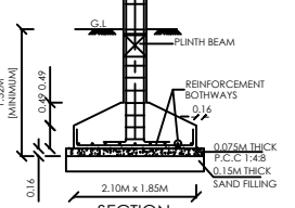
SECTION 1.85
