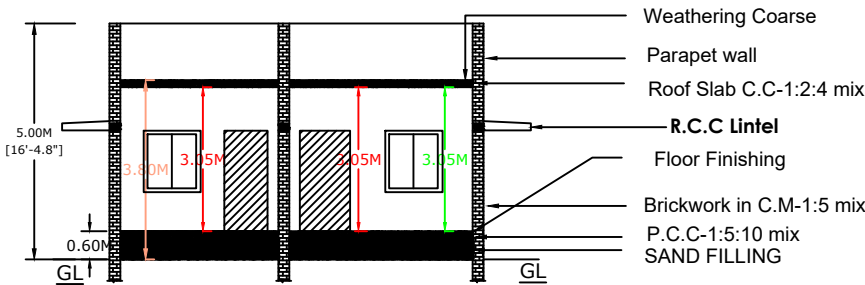
SECTION ON XX
