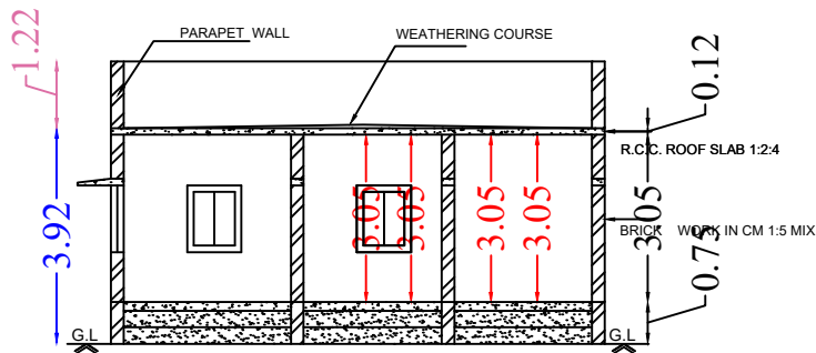
Section on-"AA"
