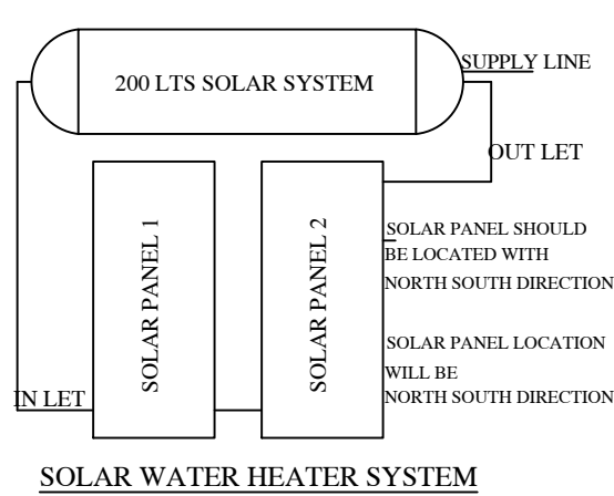
SOLAR WATER HEATER SYSTEM
