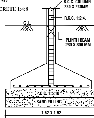
FOUNDATION DETAIL
