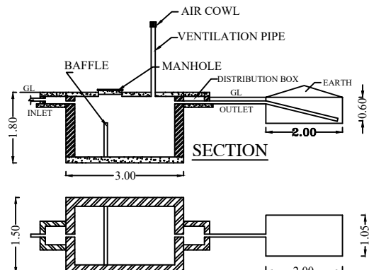
SEPTIC TANK DISPERSION TRENCH
