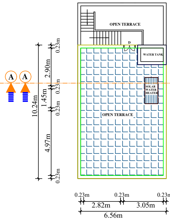
TERRACE PLAN
