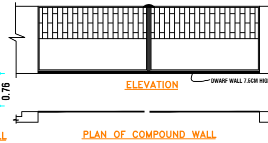
PLAN OF COMPOUND WALL
