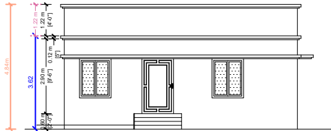
FRONT ELEVATION
