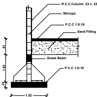
COLUMN DETAIL
