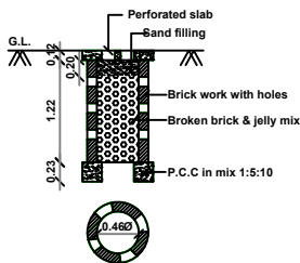
PERCOLATION PIT FOR 30 Sq. m. (Scale:- 1:50)
