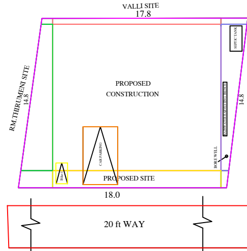
SITE PLAN
