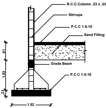
COLUMN DETAIL
