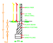
COMPOUND WALL DETAIL
