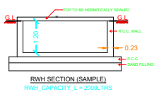
RWI SECTION (SAMPLE) RWI_CAPACITY_L = 2000 LTRS
