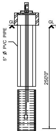
BOREWELL DETAILS
