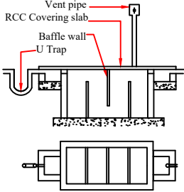
SEPTIC TANK
