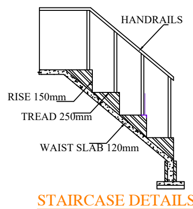
STAIRCASE DETAILS
