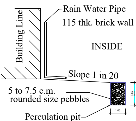
RAIN WATER HARVESTING PERCOLATION PIT RWH_CAPACITY_L=2000LTRS
