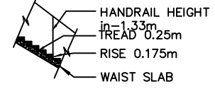
STAIRCASE DETAILS
