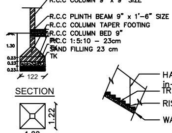
COLUMN DETAILS
