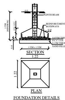
FOUNDATION DETAILS
