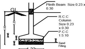
FOUNDATION DETAILS
